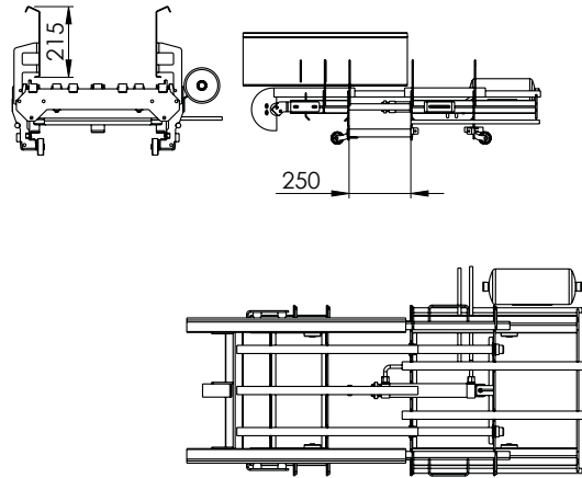
Reversible conveyor for fire doors with 215 mm sides, driven together
