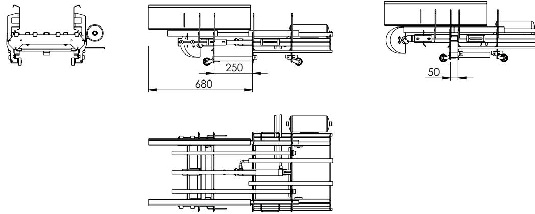
Reversible conveyor for fire doors with 160 mm sides, driven apart
